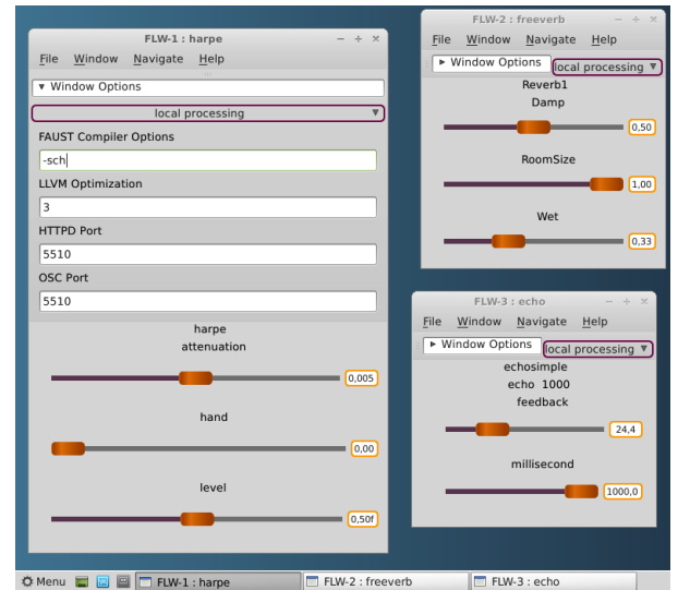
Figure 13: FaustLive's environment
